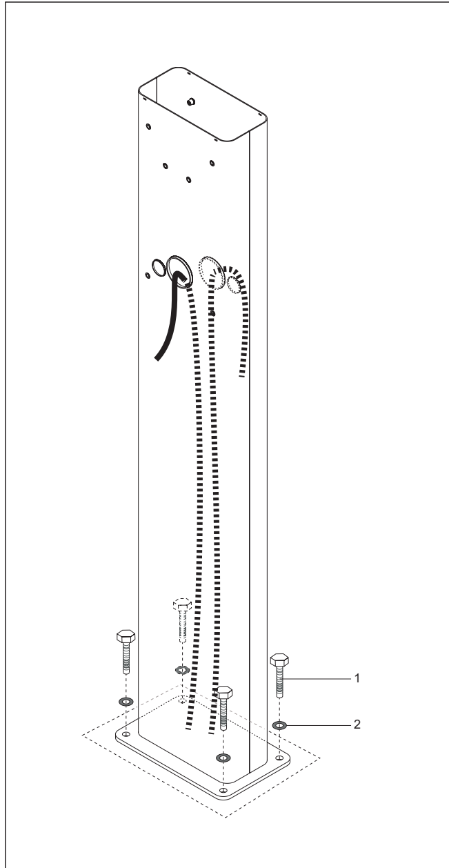
Fig. 03: Final mounting
