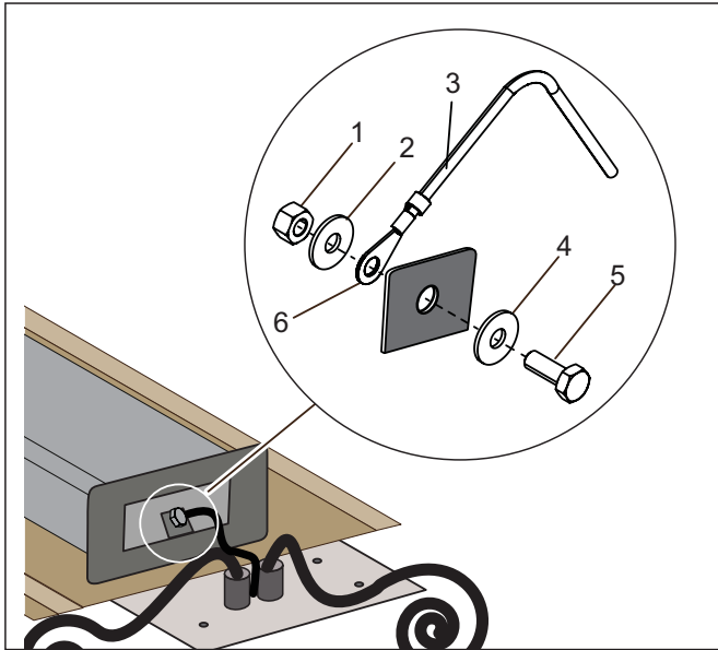
Fig. 01: Ground connection
